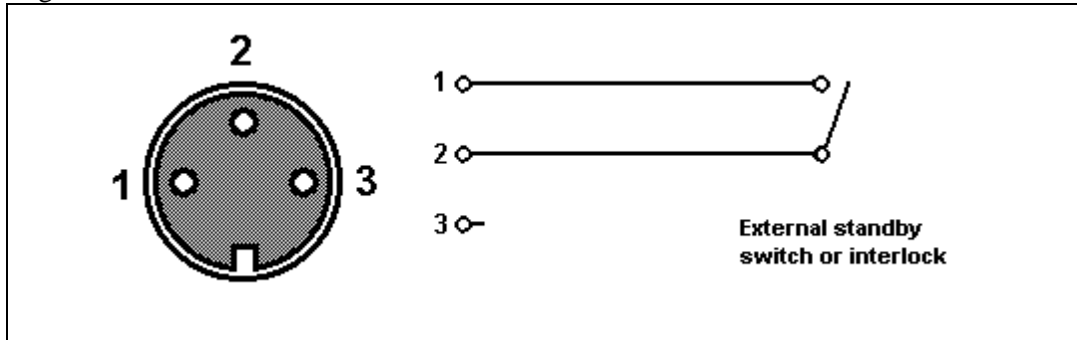
Fig 1 Interlock connector
